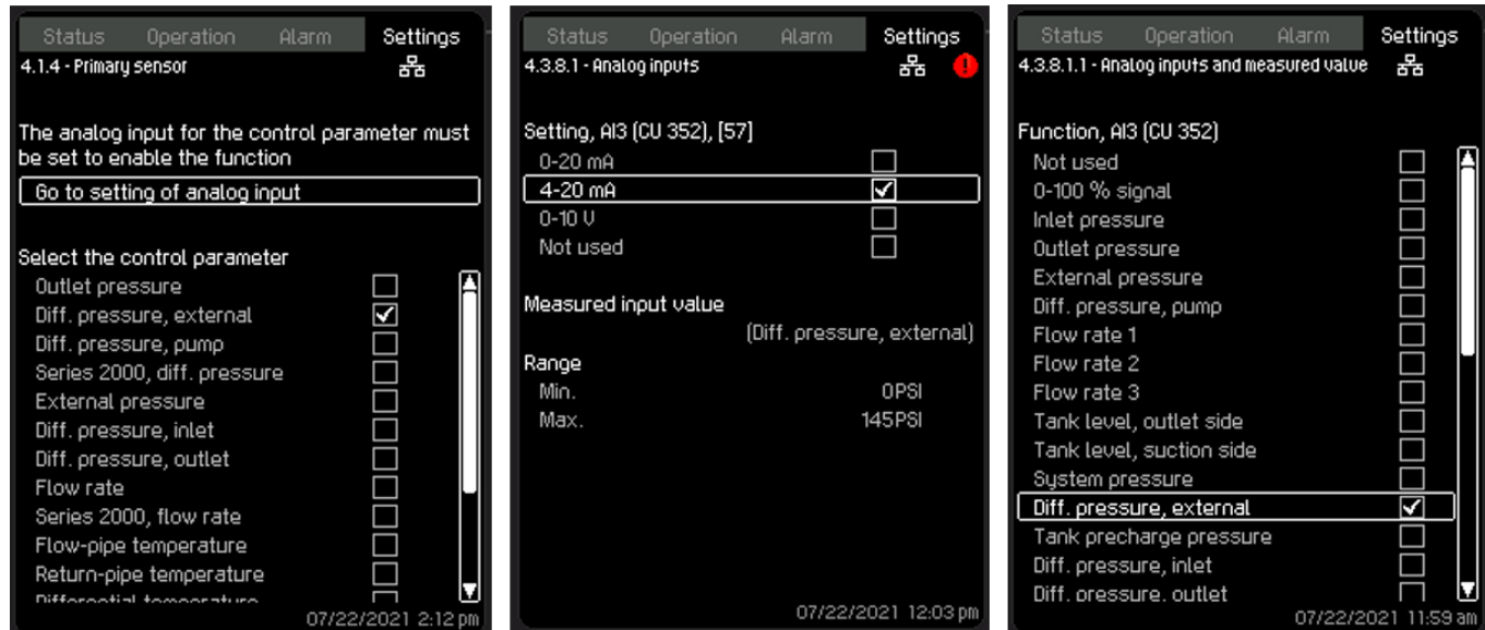
Figure 9: Setting up remote dP as primary sensor
