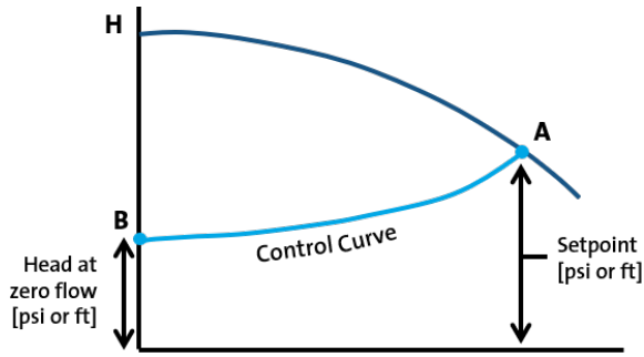
Figure 3: Control curve for pump mounted sensor with quadratic control
