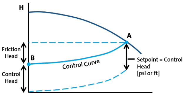
Figure 2: Control curve for remote dP
