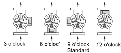
Fig. 59 Possible terminal box positions
