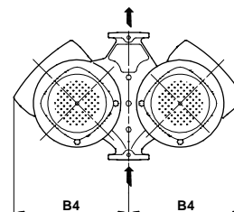
Fig. 60 Terminal box positions of TPE3 D pumps
