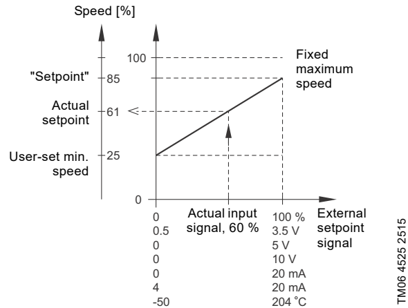
Fig. 38 Example of setpoint influence with constant curve
